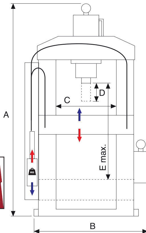
Moveable Cylinder
